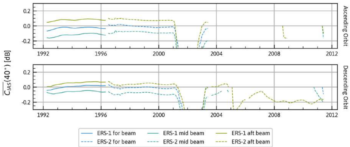
Figure 2.6: Computed intra-calibration coefficient at 40 degrees incidence angle for ERS-1 and ERS-2 over time. Note the breakdown in calibration parameter calculation for ERS-2 after 2003.
