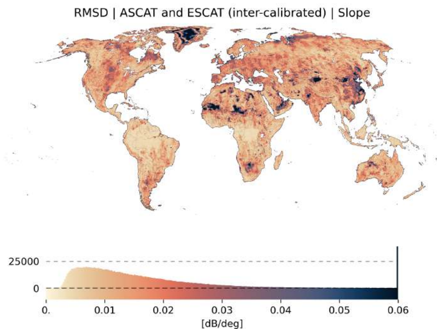
Figure 3.24: Global map of root mean squared differences (RMSD) between the slope climatologies of inter-calibrated ESCAT and ASCAT data.
