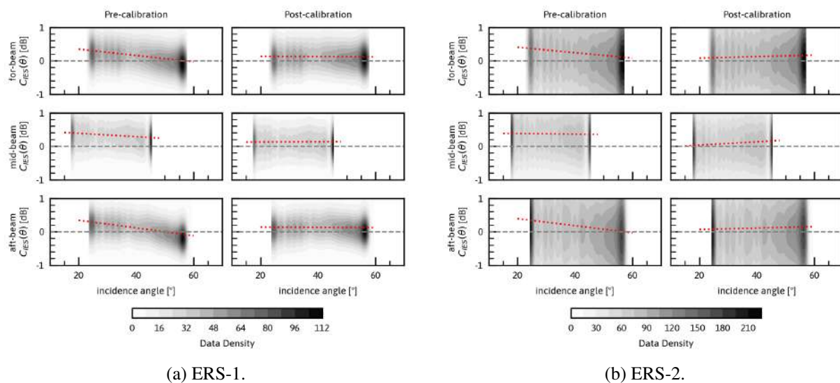
Figure 2.32: Inter-calibration coefficients (dashed line) correcting (a) ERS-1 and (b) ERS-2 against MetOp-A plotted over incidence angle, before and after inter-calibration has been applied to the backscatter data. The density of observations is shaded in the background. (Validation regions; ascending orbits)
