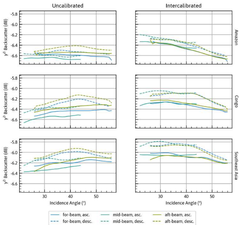
Figure 2.30: Average \gamma^0 backscatter over incidence angle for each azimuth configuration of ERS-2, before and after intercalibration, for the natural target regions. Inter-beam alignment is improved.
