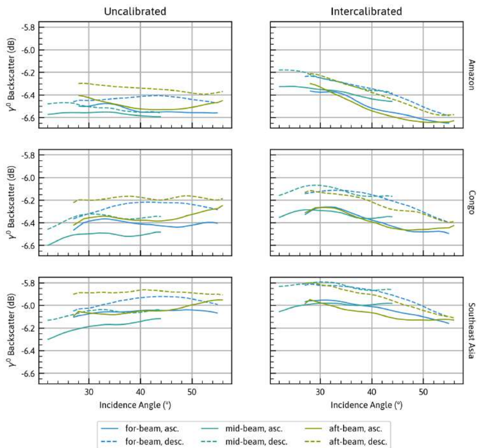
Figure 2.29: Average \gamma^0 backscatter over incidence angle for each azimuth configuration of ERS-1, before and after intercalibration, for the natural target regions. Inter-beam alignment is improved.
