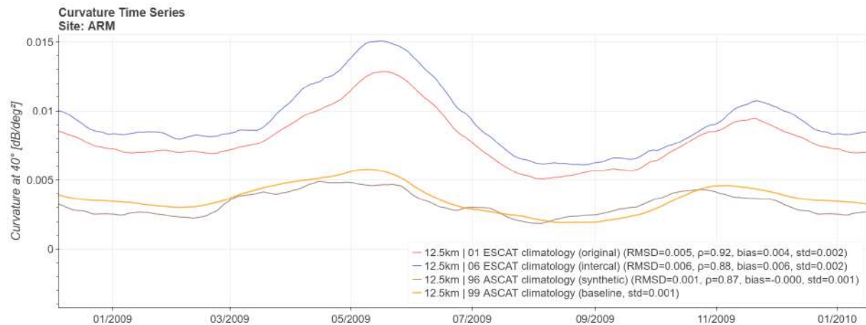
Figure 3.13: Time series of curvature for 2009 at the ARM station in Oklahoma, USA. Comparison between original ASCAT (bold orange, v99), synthetic ESCAT (brown, v96), original ESCAT (red, v01), and inter-calibrated ESCAT data (dark blue, v06).
