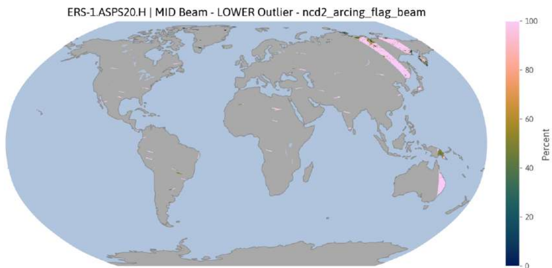
Figure A.33: Lower outliers (in percent) that have been flagged by the node confidence data field “Arcing flag” for the Mid beam in ERS-1.ASPS20.H.
