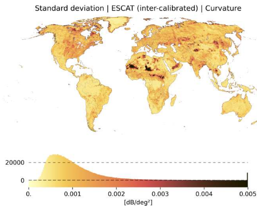
Figure 3.36: Global map of standard deviations (std) of the curvature climatologies of inter-calibrated ESCAT data.
