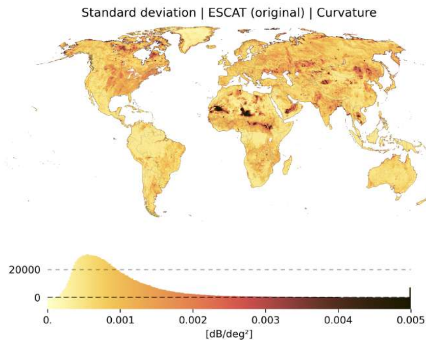
Figure 3.35: Global map of standard deviations (std) of the curvature climatologies of original ESCAT data.
