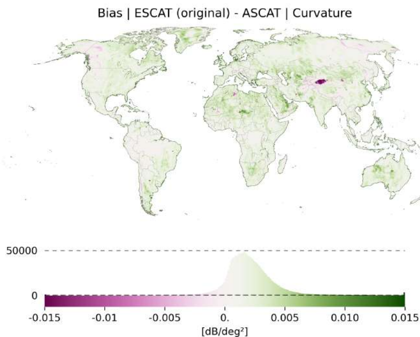
Figure 3.28: Global map of biases between the mean curvature climatologies of original ESCAT and ASCAT data. Positive (green) values indicate higher mean curvatures in the original ESCAT data compared to ASCAT.
