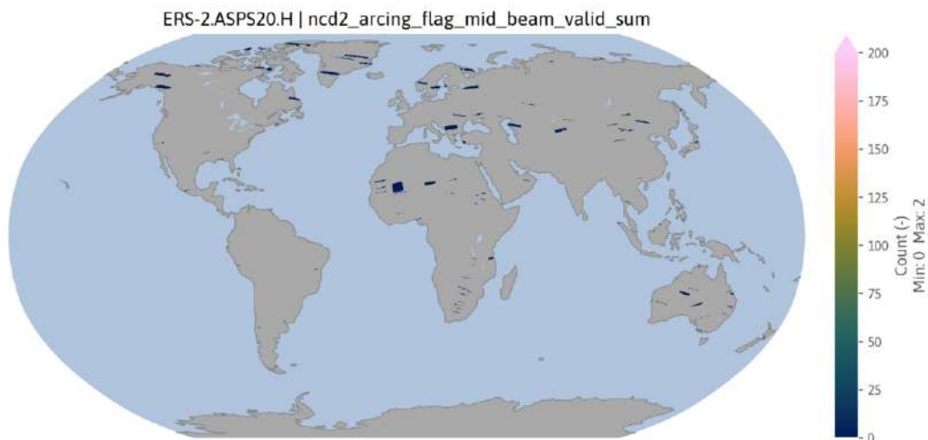
Figure 1.27: Mid beam arcing flag for dataset ERS-2.ASPS20.H.
