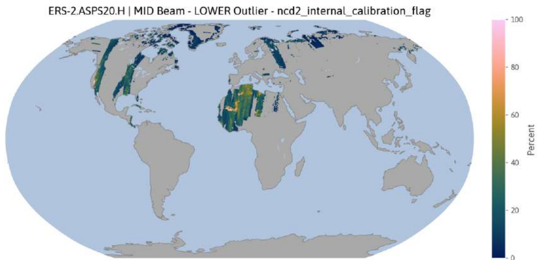
Figure A.81: Lower outliers (in percent) that have been flagged by the node confidence data field “Internal calibration flag” for the Mid beam in ERS-2 . ASPS20 . H.
