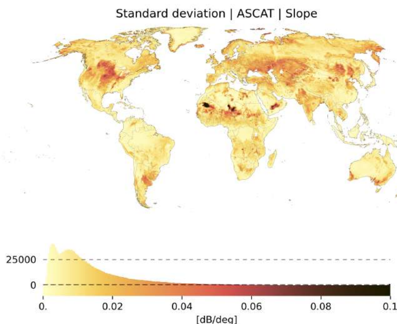
Figure 3.25: Global map of standard deviations (std) of the slope climatologies of ASCAT data.
