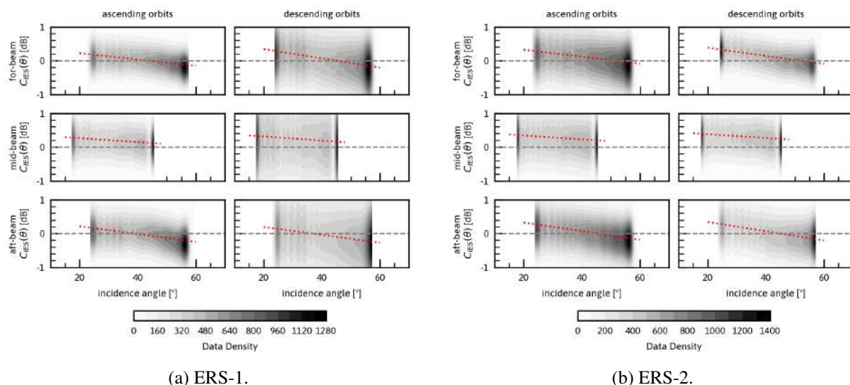
Figure 2.31: Inter-calibration coefficients (dashed lines) correcting (a) ERS-1 and (b) ERS-2 against MetOp-A plotted over incidence angle for all azimuth configurations. The density of observations is shaded in the background. (Calibration regions: Amazon and Congo rainforests)
